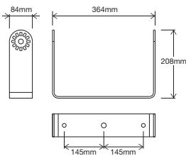
Fixed Plant Bracket MBR-CP56-FPB
