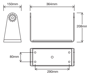
Mobile Plant Bracket (Optional) MBR-CP56-MPB
